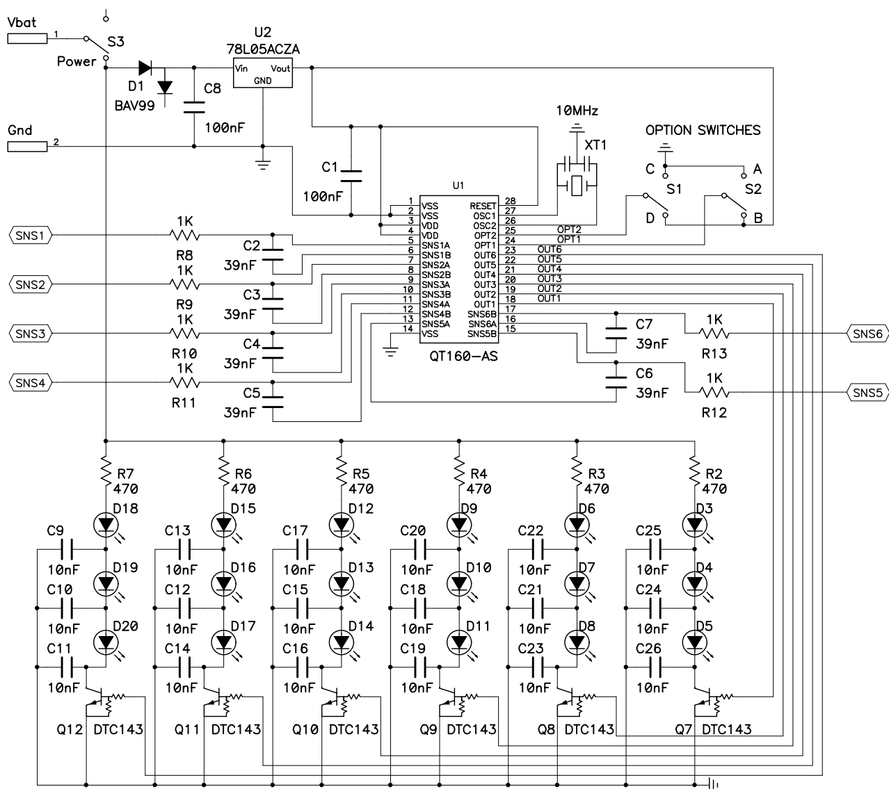
Figure 1 - E160 Schematic
