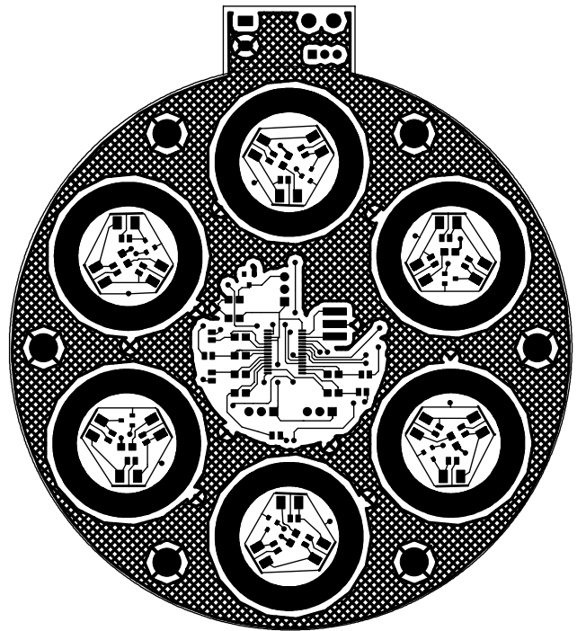
Figure 3 - PCB Component Layer
